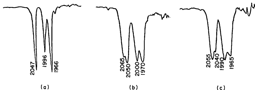
Fig. 4. Infrared spectral changes for a solution of [\text{Ru}(\text{PhCOO})(\text{CO})_2\text{PhCOOH}]_2 (5a) and DMAD in toluene: (a) at ambient temperature; (b) after 1 h reflux; (c) after addition of \text{PPh}_3 .
