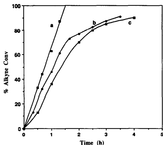
Fig. 2. Rates of reaction of 4-fluorobenzoic acid and 4-octyne with the following catalysts: a. [\text{Ru}(4\text{-FC}_6\text{H}_4\text{COO})(\text{CO})_2(4\text{-FC}_6\text{H}_4\text{COOH})_2] ; b. [\text{Ru}(4\text{-FC}_6\text{H}_4\text{COO})(\text{CO})_3]_2 ; c. \text{Ru}_3(\text{CO})_{12} . Conditions: [\text{4-octyne}] = [\text{p-FC}_6\text{H}_4\text{COOH}] = 0.2 \text{ M} ; [\text{Ru}] = 0.012 \text{ M} ; internal standard [\text{naphthalene}] = 0.08 \text{ M} in toluene in a closed reactor at 145^\circ\text{C} .
