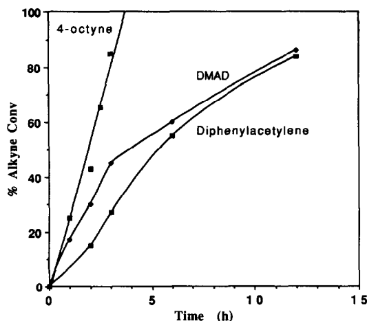
Fig. 1. Rates of reaction of benzoic acid with various alkynes. Conditions: [alkyne] = [PhCOOH] = 0.2 M; [(\text{Ru}(\text{PhCOO})(\text{CO})_2)_2 \cdot \text{PhCOOH}]_2 (5a) = 0.006 M; internal standard [ cis -Decalin] = 0.08 M in toluene at 110°C.
