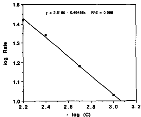
Fig. 3. Log plot of the rate of reaction of benzoic acid and 4-octyne as a function of the concentration of [\text{Ru}(\text{PhCOO})(\text{CO})_2\text{PhCOOH}]_2 (5a). Conditions: [\text{PhCOOH}] = [\text{4-octyne}] = 0.2 \text{ M} ; internal standard [\text{cis-decalin}] = 0.08 \text{ M} in toluene at 110^\circ\text{C} .
