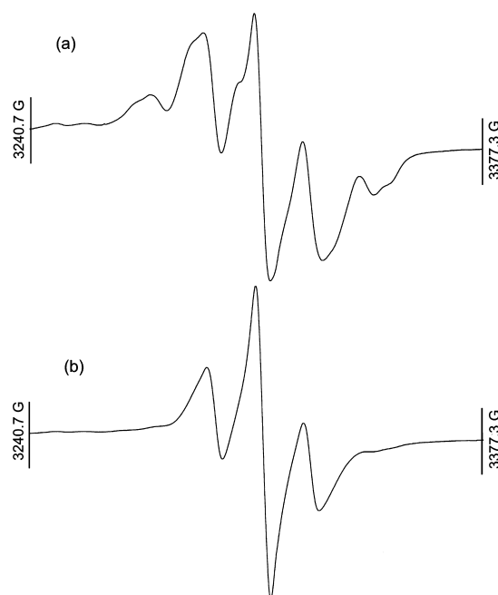
Figure 6. ESR spectrum of \gamma -irradiated 1 in \text{CF}_2\text{ClCFCl}_3 at 100 K before (a) and after (b) NIR photolysis for 1.5 h using a Corning 3962 filter. Spectrum (a) is essentially the same as the quintet observed in Figure 1 except that the additional triplet splitting is only partially resolved in this matrix. Spectrum (b) is identical in all respects to that recorded at the same temperature after \gamma -irradiation of a \text{CF}_2\text{ClCFCl}_3 solution of 4 .
