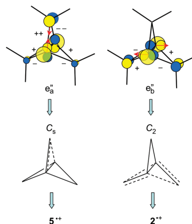
Figure 12. Schematic representation of the transition density arising from the interaction of the 2A_1 ground state with the two components of the 2E'' excited state of 1^{++} , and the weakening of bonds it induces.
