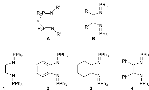
Scheme 1 Diiminophosphorane ligands.
