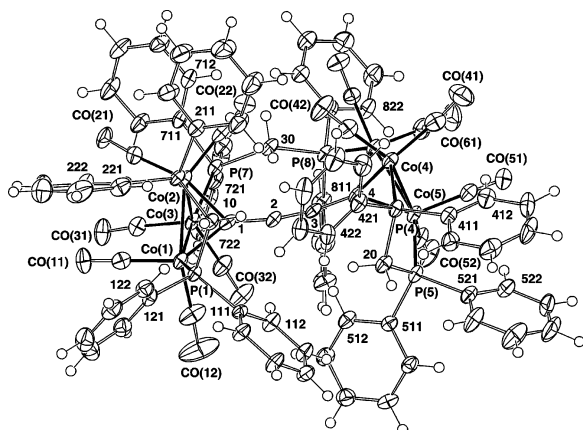
Figure 3. Plot of a molecule of \{\text{Co}_3(\mu\text{-dppm})(\text{CO})_7\}_2(\mu_3\text{-}\mu_3\text{-CC}\equiv\text{CC})(\mu\text{-dppm}) ( 7 ), showing the atom-numbering scheme. Selected distances (Å) and angles (deg): Co(1)–Co(2) = 2.4983(10), Co(1)–Co(3) = 2.4654(9), Co(2)–Co(3) = 2.4948(9), Co(4)–Co(5) = 2.4827(9), Co(4)–Co(6) = 2.5097(9), Co(5)–Co(6) = 2.4723(9), Co(1)–P(1) = 2.199(1), Co(2)–P(2) = 2.186(1), Co(3)–P(7) = 2.216(2), Co(4)–P(4) = 2.217(1), Co(5)–P(5) = 2.201(2), Co(6)–P(8) = 2.242(3), Co(1,2,3)–C(1) = 1.923(5), 1.920(4), 1.960(4), Co(4,5,6)–C(4) = 1.937(5), 1.930(4), 1.946(5), C(1)–C(2) = 1.396(7), C(2)–C(3) = 1.236(7), C(3)–C(4) = 1.387(7); Co(1,2,3)–C(1)–C(2) = 141.7(4), 129.2(4), 124.0(3), C(1)–C(2)–C(3) = 168.3(5), C(2)–C(3)–C(4) = 172.0(5), C(3)–C(4)–Co(4,5,6) = 126.1(3), 141.9(4), 127.6(3).
