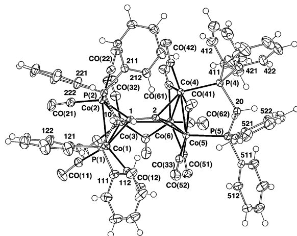
Figure 1. Plot of a molecule of Co 6 ( \mu_6 -C 2 )( \mu -dppm) 2 ( \mu -CO)(CO) 12 ( 5 ), showing the atom-numbering scheme. Selected distances (Å) and angles (deg): Co(1)–Co(2) = 2.4991(7), Co(1)–Co(3) = 2.5079(6), Co(2)–Co(3) = 2.5412(6), Co(3)–Co(6) = 2.6788(6), Co(4)–Co(5) = 2.4069(7), Co(4)–Co(6) = 2.4682(6), Co(5)–Co(6) = 2.4806(6), Co(1)–P(1) = 2.1929(9), Co(2)–P(2) = 2.2243(8), Co(4)–P(4) = 2.2348(9), Co(5)–P(5) = 2.2416(8), Co(1,2,3)–C(1) = 1.927(3), 1.873(2), 2.001(3), Co(4,5,6)–C(2) = 1.946(3), 1.938(2), 2.024(3), C(1)–C(2) = 1.367(3); Co(1,2,3)–C(1)–C(2) = 136.3(2), 141.4(2), 102.2(2), Co(4,5,6)–Co(2)–Co(1) = 138.1(2), 143.4(2), 115.7(2).
