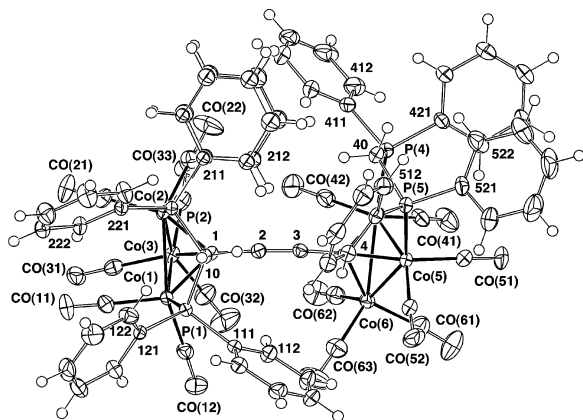
Figure 2. Plot of a molecule of \{\text{Co}_3(\mu\text{-dppm})(\text{CO})_7\}_2(\mu_3\text{-}\mu_3\text{-CC}\equiv\text{CC}) ( 6 ), showing the atom-numbering scheme. Selected distances (Å) and angles (deg): Co(1)–Co(2) = 2.4826(6), Co(1)–Co(3) = 2.4501(7), Co(2)–Co(3) = 2.4590(7), Co(4)–Co(5) = 2.4755(8), Co(4)–Co(6) = 2.4672(6), Co(5)–Co(6) = 2.4697(8), Co(1)–P(1) = 2.183(1), Co(2)–P(2) = 2.178(1), Co(4)–P(4) = 2.180(1), Co(5)–P(5) = 2.187(1), Co(1,2,3)–C(1) = 1.895(3), 1.902(3), 1.958(3), Co(4,5,6)–C(4) = 1.921(3), 1.896(4), 1.952(3), C(1)–C(2) = 1.381(5), C(2)–C(3) = 1.232(4), C(3)–C(4) = 1.370(4); Co(1,2,3)–C(1)–C(2) = 136.4(2), 135.0(2), 123.6(3), C(1)–C(2)–C(3) = 171.8(4), C(2)–C(3)–C(4) = 169.9(4), C(3)–C(4)–Co(4,5,6) = 129.4(3), 141.6(3), 123.8(3).
