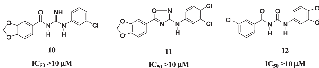
Figure 3. Effect of modifying the acylurea linker or transposing rings A and B–C.
