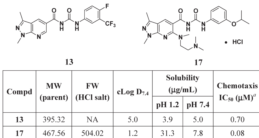
Figure 4. Structure and properties of compounds 13 and 17.
