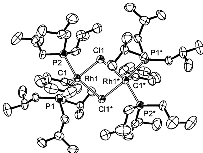
Figure 4. [\text{Rh}(\text{P}^t\text{Bu}_3)_2(\text{C}_6\text{H}_5)(\mu\text{-Cl})_2][\text{BAR}^F_4]_2 ( 4a ) (40% probability ellipsoids). The anions, minor disordered components, and hydrogen atoms have been omitted for clarity.
