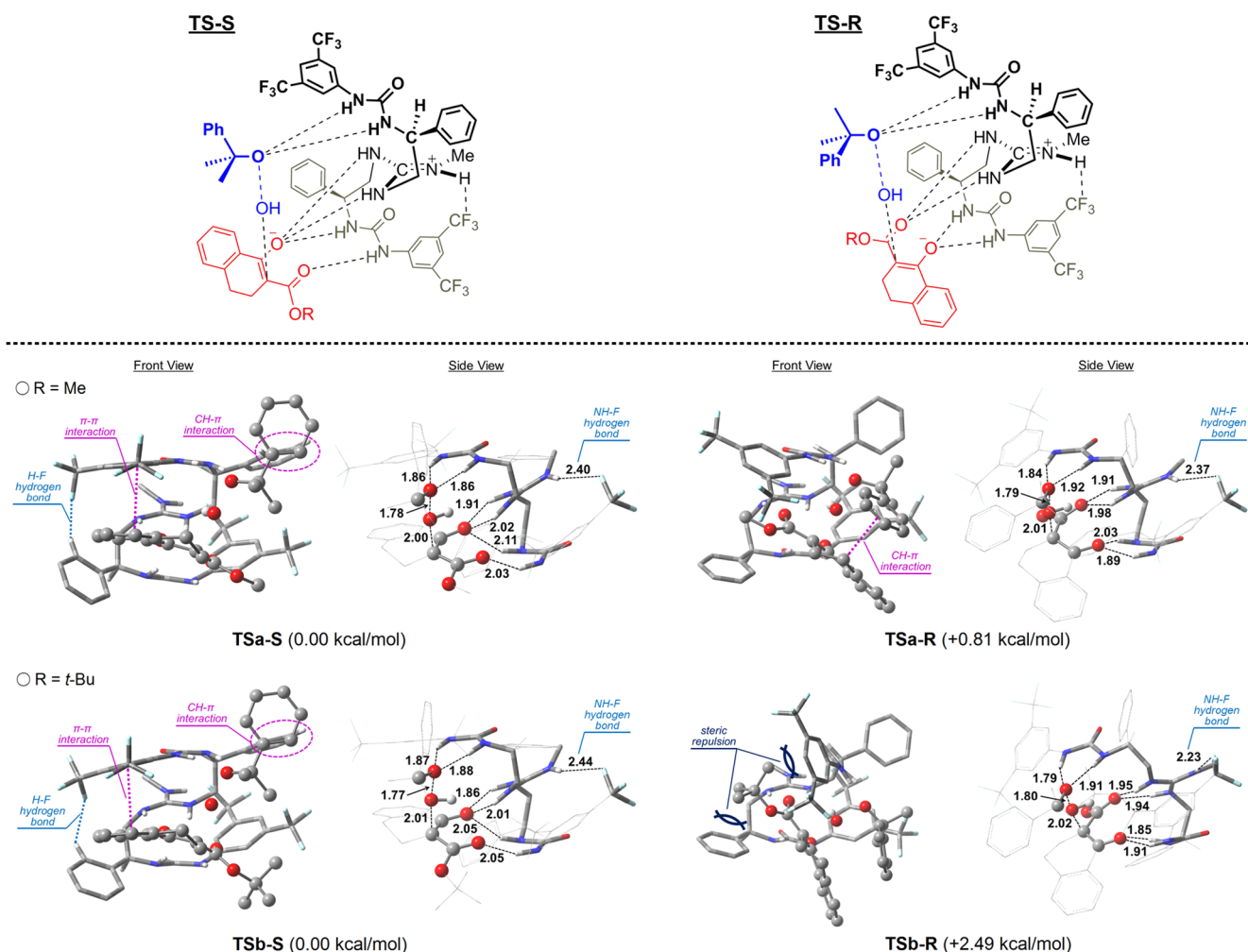
Figure 1. Schematic representations (front view) and 3D structures (bottom and side views) of TS-S and TS-R (TSa: R = Me, TSb: R = t -Bu) for 3- \beta -Ketoester enolate and CHP are indicated by ball and stick models; the catalyst is shown as a tube model; unimportant hydrogen atoms are omitted. Distances are in Å.
