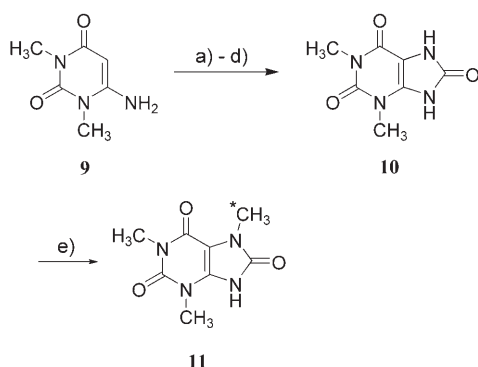
Scheme 3. a) KNO 2 , CH 3 COOH, 95%; b) Na 2 S 2 O 4 , NH 3 , 89%; c) ClCOOEt, H 2 O, 99%; d) 235 °C, neat, 89%; e) NaOH, 14 CH 3 I, acetone/H 2 O, 22%.
