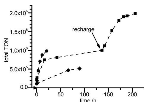
Figure 5. Kinetics of Heck-type coupling between 4-bromoacetophenone and butyl acrylate at 145 °C in DMAc. With 0.0001 mol % of 15 (○), 0.0001 mol % of 16 (◆), or 0.0001 mol % of 15 and 0.2 mol % of TBAB (■) as catalyst.
