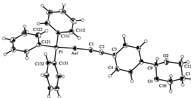
Fig. 1. Molecular geometry and atomic labeling scheme for [Au{C≡CC 6 H 4 CHO(CH 2 ) 3 O}(PPh 3 )] ( 9 ).
