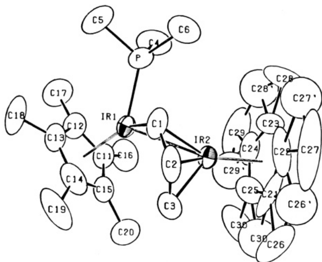
Figure 2. ORTEP diagram of 2 .
