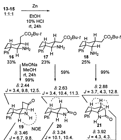
Chart 4. Reduction of a Nitro Group and Lactam Formation.
