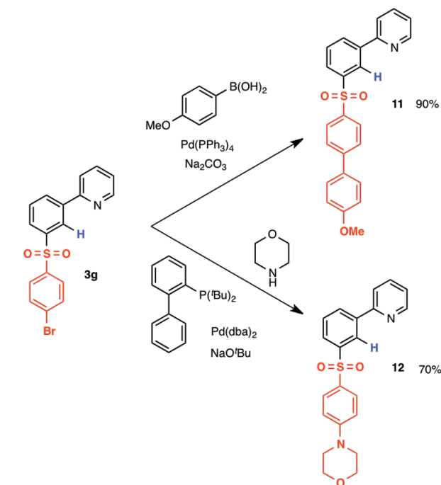
Scheme 3. Palladium-Catalyzed Cross-Coupling
