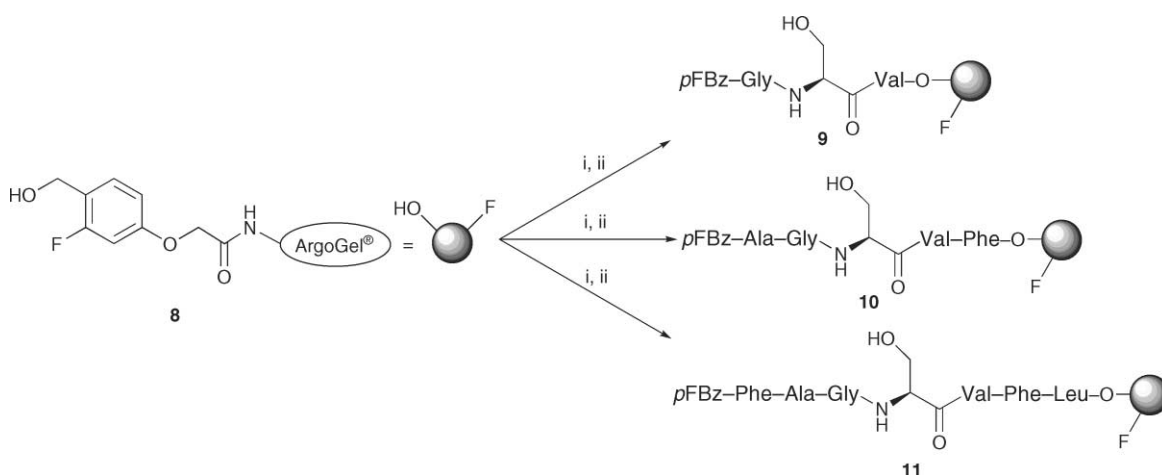
Scheme 1 Solid-phase synthesis of peptide resins 9–11 on resin 8 . Reagents and conditions: i) Fmoc-Ala-OH, Fmoc-Phe-OH or Fmoc-Leu-OH (4 equiv.), MSNT (4 equiv.), MeIm (3 or 4 equiv.), CH 2 Cl 2 , RT. ii) Peptide synthesis according to the Fmoc protocol. MSNT = 1-(mesitylenesulfonyl)-3-nitro-1,2,4-triazole, MeIm = 1-methylimidazole.
