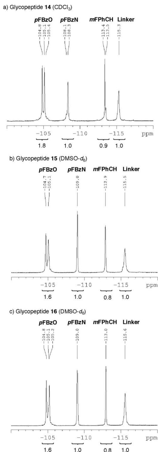
Fig. 3 ^{19}\text{F} NMR spectra of resin bound glycopeptides 14 – 16 after three identical glycosylations; (a) 90% conversion of resin 9 , (b) 80% conversion of resin 10 , (c) 80% conversion of resin 11 .
