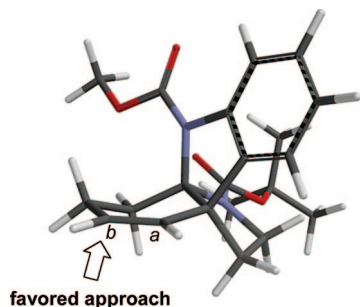
Figure 3. Proposed rationale for stereoselection in the epoxidation of alkene 27 . Model (6-31G*) of the most stable conformation of alkene 27 showing the favored approach of an oxidant to alkene carbon b .
