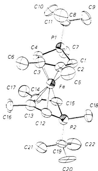
Figure 1. ORTEP view of 7 molecule I, together with the labeling scheme used. Molecule II contains atoms labeled Fe2, P3, P4, and carbon atoms C23–C44. Atoms are represented by their thermal ellipsoids scaled to enclose 50% of the electron density, and hydrogen atoms are omitted.
