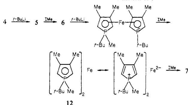
Scheme I. Possible Mechanism for the Formation of 7
