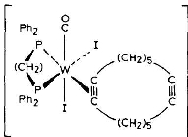
Fig. 2. Proposed structure of the complex [WI_2(CO)(dppm)(\eta^2\text{-1,8-CTDiene})] .
