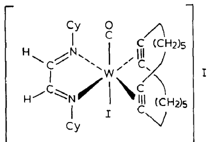
Fig. 3. Proposed structure of the complex [WI(\text{CO})(\text{CyN}=\text{CHCH}=\text{NCy})(\eta^2, \eta^{2'}\text{-1,8-CTDiene})]I \cdot \text{Et}_2\text{O} .
