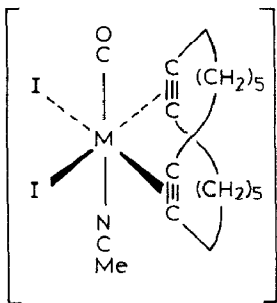
Fig. 1. Proposed structure of the complexes [\text{MI}_2(\text{CO})(\text{NCMe})(\eta^2, \eta^{2'}\text{-1,8-CTDiyne})] .
