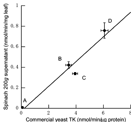
Figure 5. Correlation of activities of PGA formation in the spinach 200g supernatant and commercial yeast TK: (A) D-fructose, (B) D-fructose 6-phosphate, (C) D-xylulose 5-phosphate, and (D) hydroxypyruvate. Initial velocities of PGA formation were measured under the condition described in the Materials and Methods. Values are means \pm SD ( n = 3 ).
