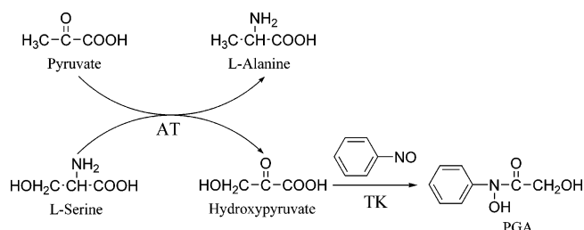
Scheme 1. Two Stages of the Mechanism for Pyruvate-Dependent Formation of PGA from NOB a
