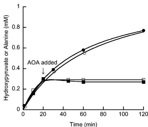
Figure 4. Hydroxypyruvate and alanine formation in transamination between pyruvate and L-serine and inhibitory effect of aminooxyacetic acid. Hydroxypyruvate formation (●) and in the addition of aminooxyacetic acid (■); Alanine formation (○) and in the addition of aminooxyacetic acid (□). The incubation was started with 10 mM pyruvate and 10 mM L-serine in the presence of dialyzed 105 000g supernatant. Aminooxyacetic acid was added at the final concentration of 0.1 mM.
