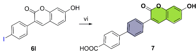
Scheme 2. Synthesis of 7 . Reagents and conditions: vi . 4-boronobenzoic acid, \text{Pd}(\text{AcO})_2 , \text{Na}_2\text{CO}_3 , EtOH, rt.
