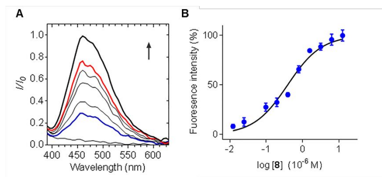
Figure 3. Fluorescence recovery of 6d in presence of MIF by 8 . A) Fluorescence spectra of 6d (100 nM) together with MIF (1.0 \mu M) increased with the addition of 8 ; B) Nonlinear regression for log concentration of 8 vs response, n=3 .
