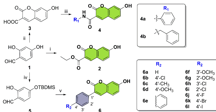
Scheme 1. Synthesis of 7-hydroxycoumarins as MIF inhibitors from 2,4-dihydroxybenzaldehyde 1 as a key precursor. Reagents and conditions: i. Diethyl malonate, piperidine, rt; ii. malonic acid, pyridine, aniline, rt; iii. EDCI, HOBt, DMF, rt; iv. TBDMSCl, imidazole, CH 2 Cl 2 , rt; v. 1) Cyanuric chloride, NMM, DMF, reflux; 2) TBAF, THF, rt.
