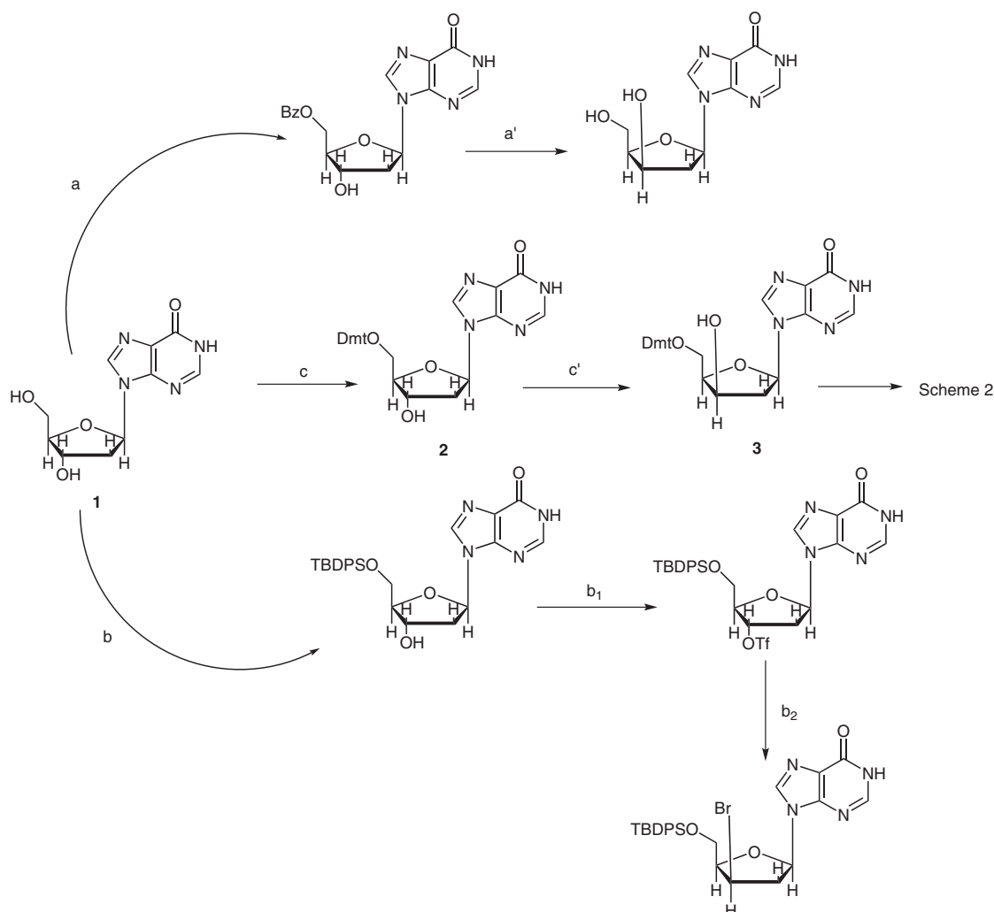
Scheme 1 Reaction conditions: (a) BzCl, py; (a') Tf 2 O, py, CH 2 Cl 2 , then H 2 O; (b) TBDPSCl, py; (b 1 ) TfCl, DMAP, CH 2 Cl 2 ; (b 2 ) NaBr, acetone, reflux; (c) DMTCl, pyridine, ; (c') 1. Dess–Martin periodinane, CH 2 Cl 2 ; 2. i -PrOH, NaBH 4 , acetone, –45 °C. Dmt = 4,4'-dimethoxytrityl.
