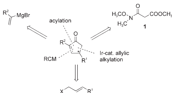
Scheme 3. Retrosynthetic concept.
