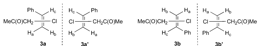
Chart 1. View of the Isomers of 3 through the Cl–Pt–Olefin Axis
