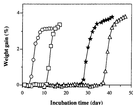
Figure 2. Effect of CA, HCA, and \alpha -Toc on autoxidation of lard at 60 °C. Antioxidants (0.4 \mu\text{mol} ) were mixed with lard (1.0 g): (○) no addition; (★) caffeic acid; (△) dihydrocaffeic acid; (□) \alpha -tocopherol. The data are representative of two experiments.
