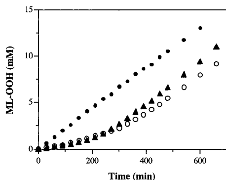
Figure 5. Effects of CA and HCA on AMVN-initiated oxidation of methyl linoleate in solution. The reaction system consisted of methyl linoleate (100 mM), AMVN (10 mM), and antioxidants (80 \mu M) in a mixture of n -hexane/2-propanol/ethanol (8:3:1, v/v/v): (○) caffeic acid; (▲) hydrocaffeic acid; (●) no addition. The data are representative of two experiments.
