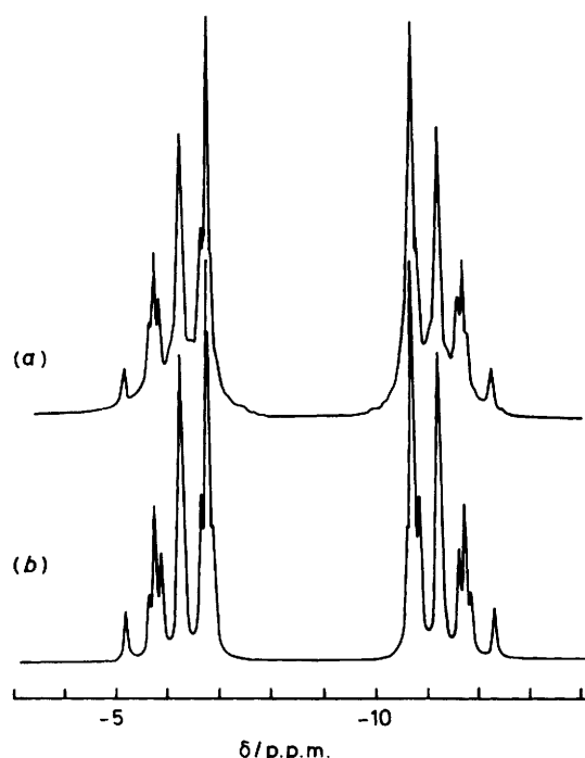
Figure 2. ^{31}\text{P}\{-^1\text{H}\} N.m.r. spectrum of [\text{Re}_2\text{Cl}_4(\text{dppm})_2(\text{CNBu}')] recorded in \text{CH}_2\text{Cl}_2\text{-CD}_2\text{Cl}_2 : (a) observed and (b) calculated. The simulation of this AA'BB' spectrum gave the following parameters: \delta_{\text{A}} = -6.39 , \delta_{\text{B}} = -11.23 p.p.m., J_{\text{AA}'} = 232.3 , J_{\text{BB}'} = 212.1 , J_{\text{AB}} = 79.7 , and J_{\text{AB}'} = 1.2 Hz
