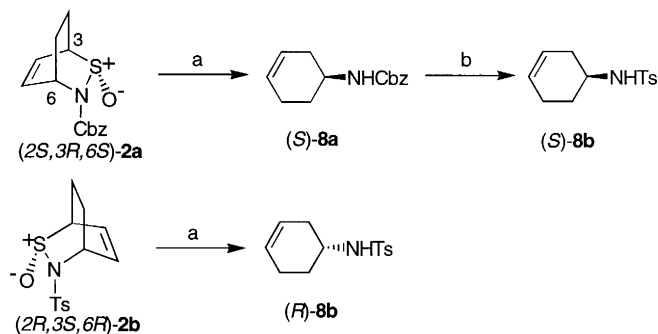
Scheme 2. (a) (i) 1.25 M aq. NaOH, rt, 14 h; (ii) 0.5 M aq. HCl, 0^{\circ}\text{C} , 10 min, 75% (Cbz), 34% (Ts); (b) (i) TMSI, MeCN, 0^{\circ}\text{C} , 30 min; (ii) MeOH, rt, 10 min; (iii) TsCl, Et 3 N, CH 2 Cl 2 , rt, 21 h, 77%
