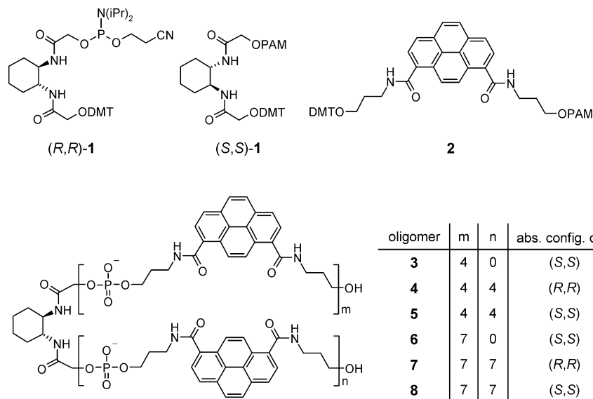
Figure 1. Oligomers 3–8 composed of achiral pyrene building blocks and a chiral 1,2-diaminocyclohexane unit as well as the respective monomeric building blocks (PAM = phosphoramidite, as shown in (R,R)-1; DMT stands for 4,4'-dimethoxytrityl).
