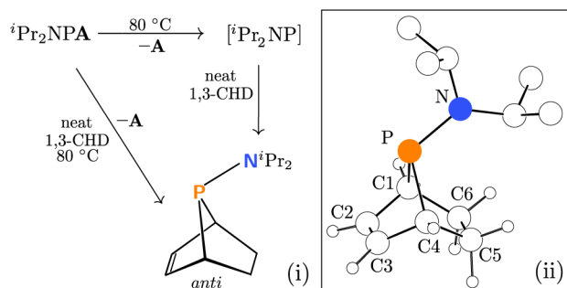
Scheme 2. (i) Thermolysis of i\text{-Pr}_2\text{NPA} in 1,3-CHD Leading to Quantitative Formation of anti - i\text{-Pr}_2\text{NPC}_6\text{H}_8 ; (ii) A Model of anti - i\text{-Pr}_2\text{NPC}_6\text{H}_8 Built and Optimized Using DFT Methods 28,29 and Visualized Using PLATON 21a
