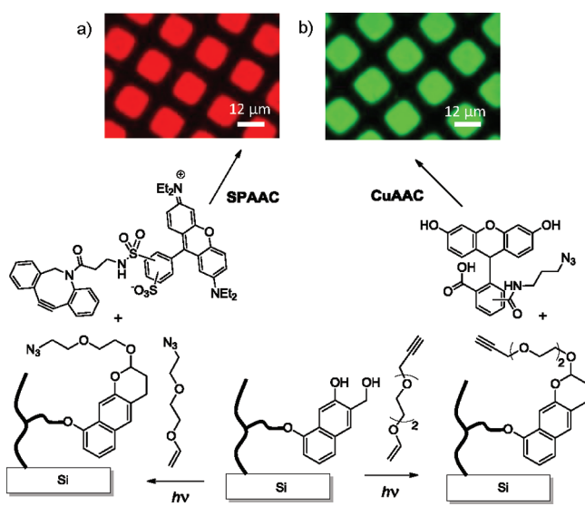
Scheme 4. Sequential Click Functionalization: Photo-Diels–Alder Surface Patterning Followed by Azide–Alkyne Click Immobilization of Fluorescent Dyes via (a) SPAAC of ADIBO–Rhodamine B on an Azide-Derivatized Surface and (b) CuAAC of Azidofluorescein
