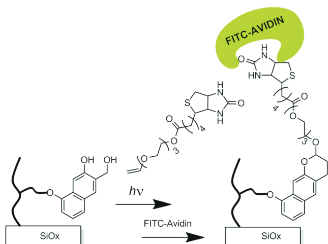
Scheme 5. Diels–Alder Photoclick Patterning of FITC–Avidin on a Poly(NQMP-4VB) Surface
