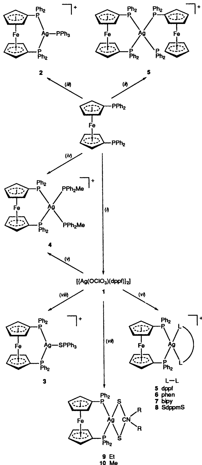
Scheme 1 (i) \text{AgClO}_4 ; (ii) 0.5 \text{ AgClO}_4 ; (iii) [\text{Ag}(\text{OCIO}_3)(\text{PPh}_3)] ; (iv) 2 [\text{Ag}(\text{OCIO}_3)(\text{PPh}_2\text{Me})] ; (v) 2 \text{ PPh}_2\text{Me} ; (vi) dppf, phen, bipy or SdppmS; (vii) \text{Na}(\text{S}_2\text{CNET}_2) or \text{Na}(\text{S}_2\text{CNMe}_2) ; (viii) \text{SPPH}_3
