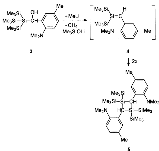
Scheme 1. Generation and head-to-tail cyclodimerization of the transient silene 4 .
