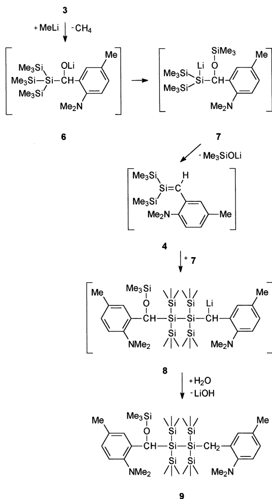
Scheme 2. Generation of the silene 4 by a sila-Peterson reaction and addition of the precursor lithium silanide 7 to the \text{Si}=\text{C} bond.
