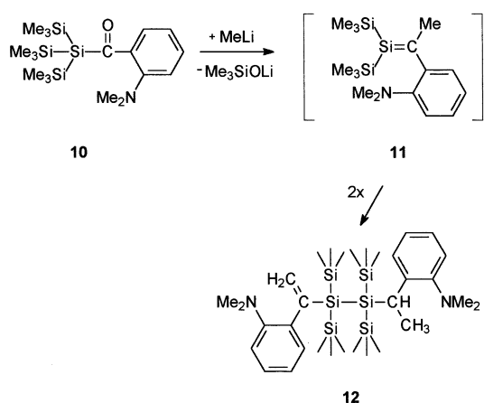
Scheme 3. Generation of the transient silene 11 and its spontaneous head-to-head reaction affording the linear dimer 12 .
