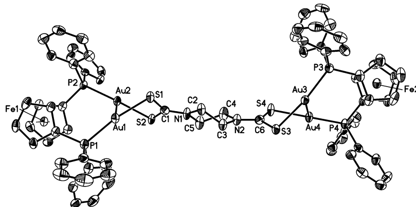
Figure 1. Molecular structure of the dication in [(\text{dppf})\text{Au}_2](\text{S}_2\text{CNC}_4\text{H}_8\text{NCS}_2)(\text{PF}_6)_2 ( 3 ). Selected bond lengths (Å) and angles (deg): Au1–P1 = 2.268(2), Au1–S1 = 2.324(2), Au1–Au2 = 3.0072(4), Au2–P2 = 2.273(2), Au2–S2 = 2.323(2), Au3–P3 = 2.268(2), Au3–S3 = 2.336(2), Au3–Au4 = 3.0368(4), Au4–P4 = 2.267(2), Au4–S4 = 2.3220(19), S1–C1 = 1.733(8), S2–C1 = 1.743(9), S3–C6 = 1.727(9), S4–C6 = 1.739(9), N1–C1 = 1.307(10), N2–C6 = 1.325(11), P1–Au1–S1 = 168.16(8), P2–Au2–S2 = 171.72(8), P3–Au3–S3 = 170.40(8), P4–Au4–S4 = 167.05(8), S1–C1–S2 = 123.9(5), S3–C6–S4 = 124.6(5).
