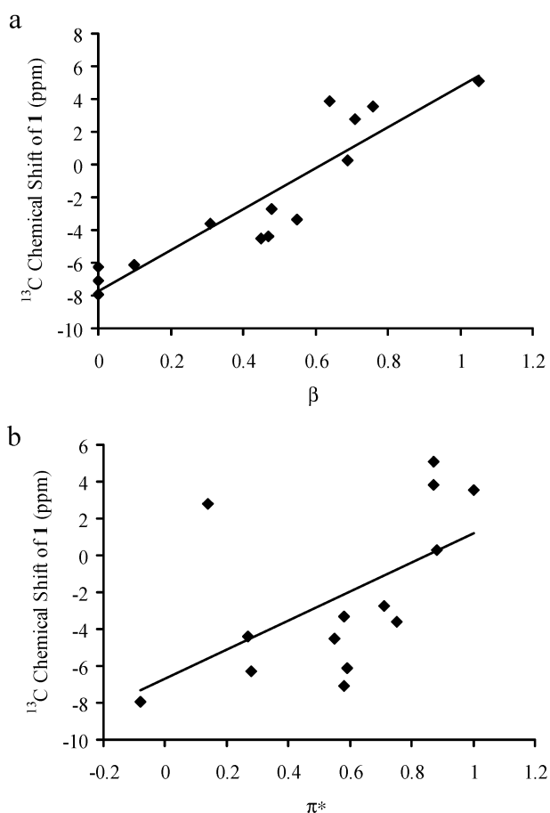
FIGURE 5. The \alpha -carbon ^{13}\text{C} NMR shift of 1 as a function of Taft and Kamlet's solvatochromatic parameters: (a) \beta and (b) \pi^* . 17–20
