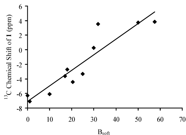
FIGURE 6. The \alpha -carbon ^{13}\text{C} NMR shift of 1 as a function of Laurence's B_{\text{soft}} values. 4
