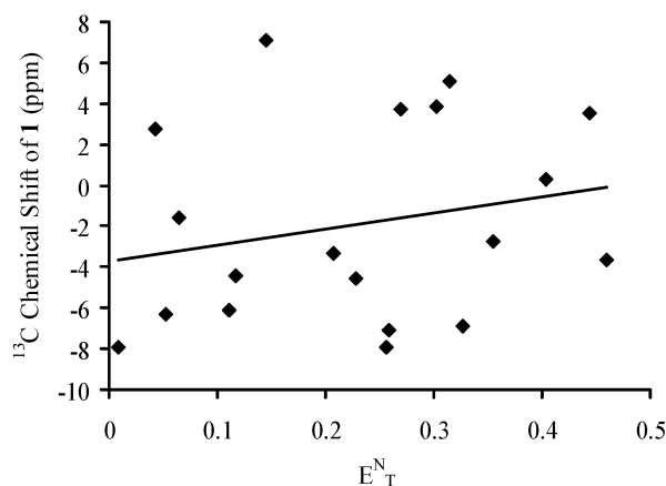
FIGURE 4. The \alpha -carbon ^{13}\text{C} NMR shift of 1 as a function of Reichardt's normalized E_{\text{T}}^{\text{N}} polarity model. 16
