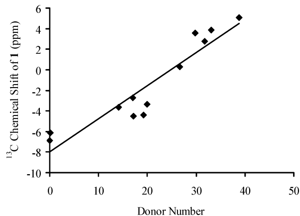
FIGURE 3. The \alpha -carbon 13 C NMR shift of 1 as a function of Gutmann's donor numbers. 15
