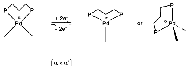
Scheme 3. Different coordination modes of dppp to \text{Pd}(\text{II}) and \text{Pd}(0) .
