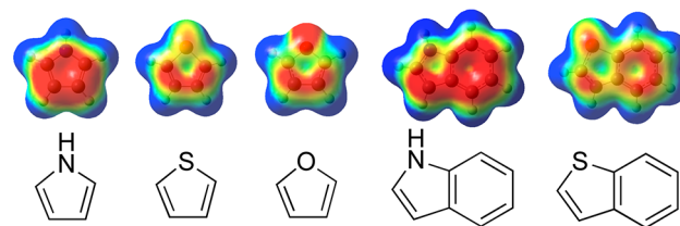
Figure 5. Electrostatic potentials (above) plotted onto electron density isosurfaces (isoval = 0.004) of unbound heterocycles (below). Red represents a potential energy lower or equal to -0.02 hartree (electron-rich), and blue a potential energy higher or equal to +0.02 hartree (electron-poor).
