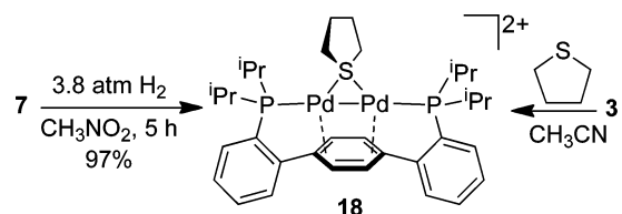
Scheme 3. Hydrogenation and Direct Routes to Tetrahydrothiophene Adduct 18
