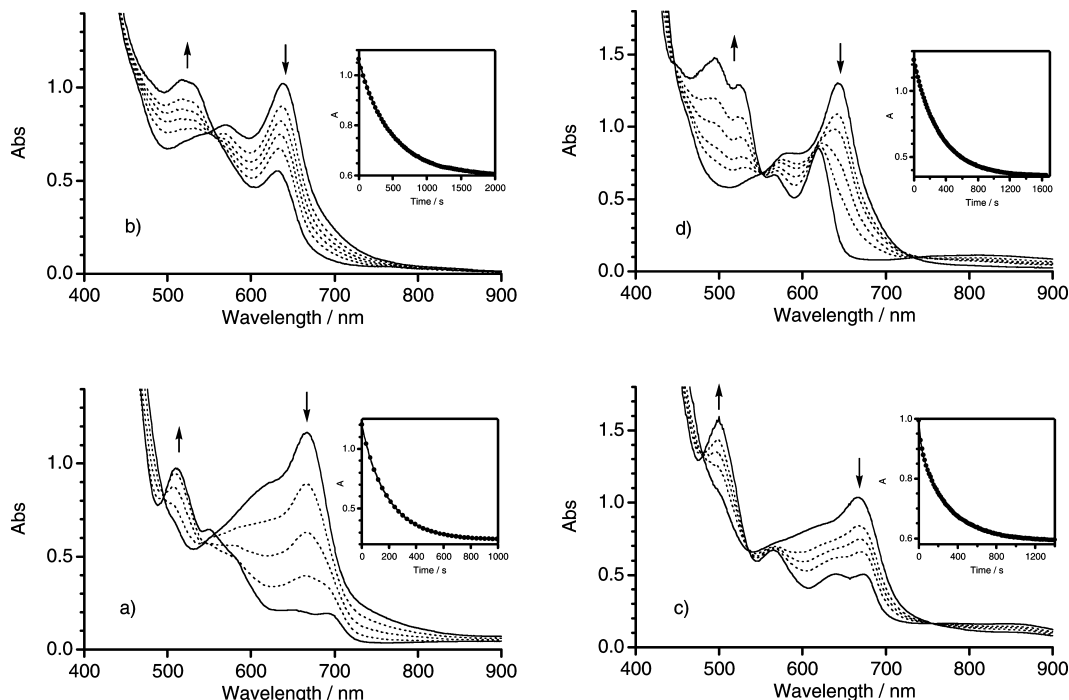
Figure 8. UV-visible absorption spectral change for the reactions of (a) [(\text{TMP}^{++})\text{Fe}^{\text{IV}}\text{O}(\text{Im})](\text{NO}_3) , (b) [(\text{TMTMP}^{++})\text{Fe}^{\text{IV}}\text{O}(\text{Im})](\text{NO}_3) , (c) (\text{TMP}^{++})\text{Fe}^{\text{IV}}\text{O}(3\text{-F-4-NO}_2\text{-PhO}) , and (d) (\text{TMTMP}^{++})\text{Fe}^{\text{IV}}\text{O}(3\text{-F-4-NO}_2\text{-PhO}) with cyclooctene ( 2.5 \times 10^{-2} M) in dichloromethane at -80^\circ\text{C} . Sample concentration = 1.0 \times 10^{-4} M in 1 cm path length cell. Insets; time dependence of the absorptions at (a) 667 nm, (b) 639 nm, (c) 667 nm, and (d) 643 nm.
