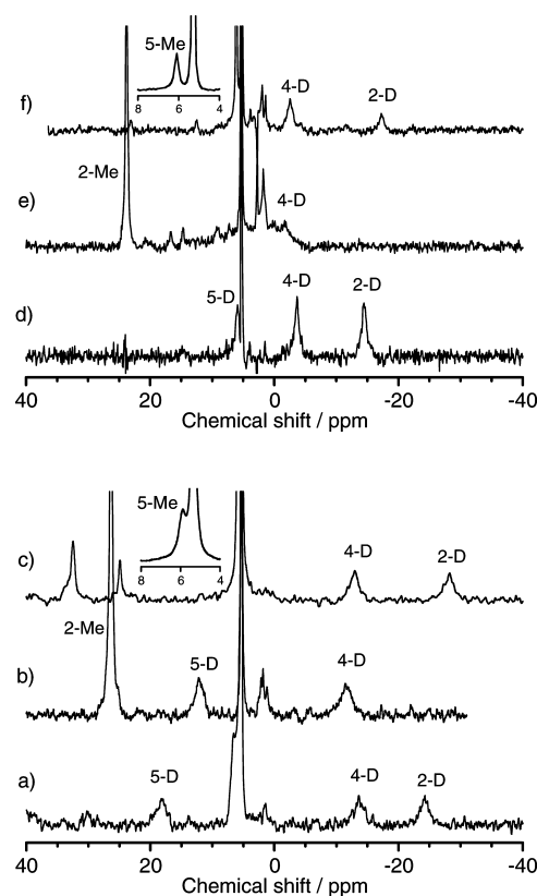
Figure 6. ^2\text{H} NMR spectra of (a) (\text{TMP}^{++})\text{Fe}^{\text{IV}}\text{O}(\text{Im-}d_4)(\text{ClO}_4) , (b) (\text{TMP}^{++})\text{Fe}^{\text{IV}}\text{O}(2\text{-MeIm-}d_6)(\text{ClO}_4) , (c) (\text{TMP}^{++})\text{Fe}^{\text{IV}}\text{O}(5\text{-MeIm-}d_6)(\text{ClO}_4) , (d) (\text{TMTMP}^{++})\text{Fe}^{\text{IV}}\text{O}(\text{Im-}d_4)(\text{ClO}_4) , (e) (\text{TMTMP}^{++})\text{Fe}^{\text{IV}}\text{O}(2\text{-MeIm-}d_6)(\text{ClO}_4) , and (f) (\text{TMTMP}^{++})\text{Fe}^{\text{IV}}\text{O}(5\text{-MeIm-}d_6)(\text{ClO}_4) in dichloromethane. Temperature; (a–c) at -60\text{ }^\circ\text{C} and (d–f) at -80\text{ }^\circ\text{C} .
