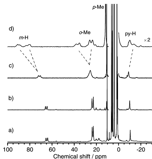
Figure 5. ^1\text{H} NMR spectra of (\text{TMP}^{++})\text{Fe}^{\text{IV}}\text{O}(\text{L})(\text{ClO}_4) in dichloromethane- d 2 at -60\text{ }^\circ\text{C} . (a) L = Im, (b) L = 5-MeIm, (c) L = 2-MeIm, (d) L = 2-MeIm at -90\text{ }^\circ\text{C} .
