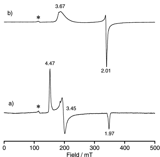
Figure 7. EPR spectra of (a) [(P ++ )Fe IV O(2-MeIm)](ClO 4 ) at 4K. (a) P = TMP, in dichloromethane-toluene (5:1), (b) P = TMTMP, in dichloromethane-propionitrile (5:1). Signals denoted by asterisks are due to [(TMP)Fe III (2-MeIm)](ClO 4 ) and [(TMTMP)Fe III (2-MeIm)](ClO 4 ).
