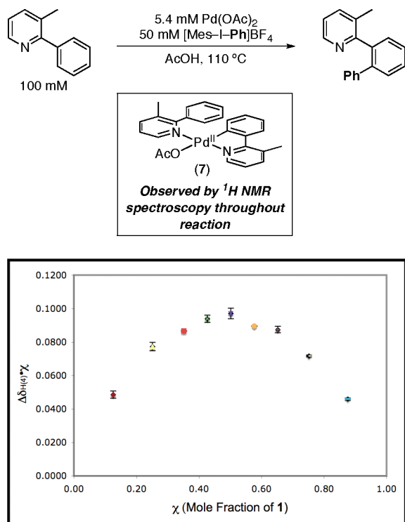
Figure 4. Job plot of \Delta\delta_{\text{H}(4)} \cdot \chi (mole fraction of substrate) versus \chi at 110 °C.
