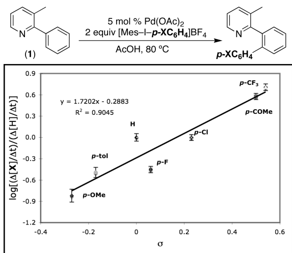
Figure 6. Hammett plot for Pd-Catalyzed C–H arylation of 1 with [\text{Mes}-\text{I}-\text{Ar}]\text{BF}_4 .
