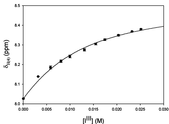
Figure 5. \delta_{\text{H}(4)} as a function of [\text{I}^{\text{III}}] at 110 °C. The line depicts a nonlinear least-squares fit to a 1:1 binding model, which showed that K_{\text{eq}} = 111 \pm 18 \text{ M}^{-1} .
