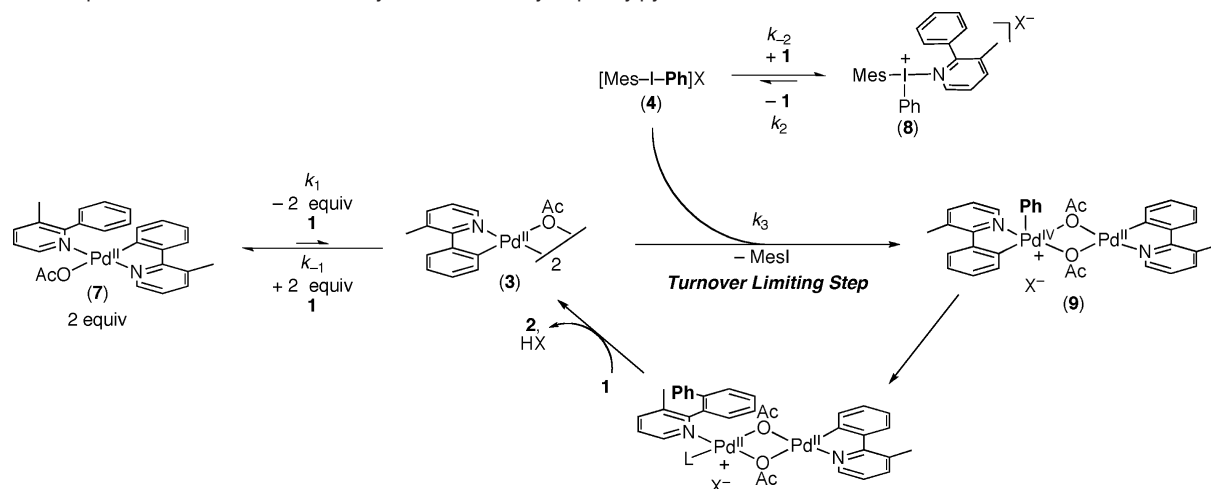
Scheme 3. Proposed Mechanism for C–H Arylation of 3-Methyl-2-phenylpyridine
