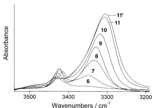
Figure 1. FT-IR absorption spectra in the 3500–3200 \text{cm}^{-1} region for the C-terminal short sequences Z-Ala-Lol ( 6 ), Boc-Glu(OMe)-Ala-Lol ( 7 ), Z-Aib-Glu(OMe)-Ala-Lol ( 8 ), Z-(Aib) 2 -Glu(OMe)-Ala-Lol ( 9 ), Boc-Glu(OMe)-(Aib) 2 -Glu(OMe)-Ala-Lol ( 10 ), and Boc-[Glu(OMe)] 2 -(Aib) 2 -Glu(OMe)-Ala-Lol ( 11 ) of peptide a in \text{CDCl}_3 solution. Peptide concentration: 1 mM. Spectrum 11' is the spectrum of the hexapeptide at 10 mM peptide concentration.
