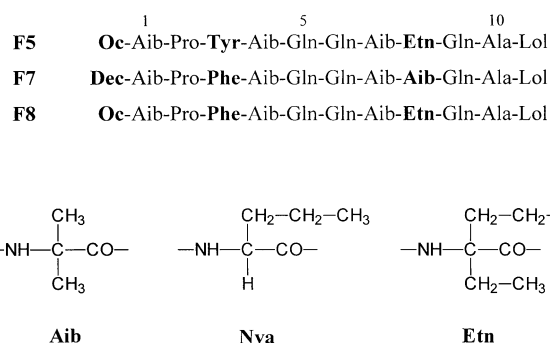
Scheme 1. Amino acid sequences of the lipopeptaibol metabolites LP237-F5, -F7, and -F8. All the \alpha -amino acids and the 1,2-amino alcohol have the S configuration. At the N-terminal acyl moiety and at positions 3 and 8, variations in the sequence are indicated in bold. The chemical formulae of Nva and the two Ca -tetrasubstituted \alpha -amino acids are also shown. Aib = \alpha -aminoisobutyric acid, Dec = n -decanoyl, Etn = Ca -ethylnorvaline, Lol = leucinol, Nva = norvaline, Oc = n -octanoyl.
