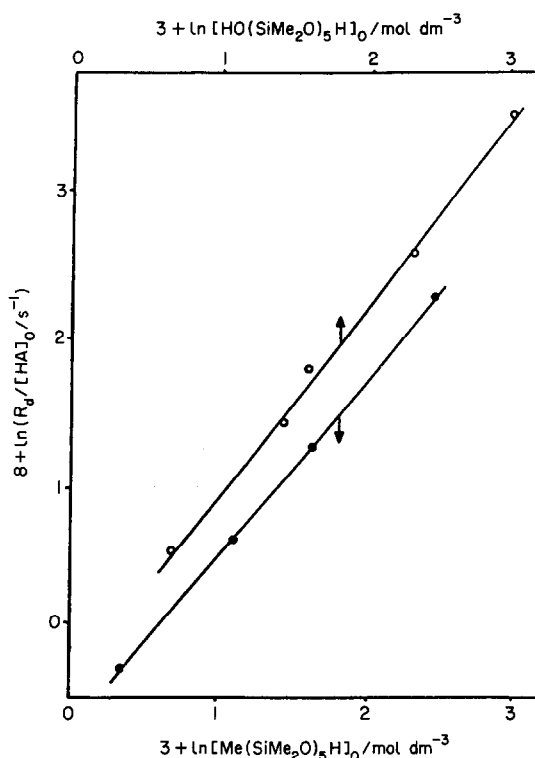
Fig. 5. Dependence of the initial rate on the initial oligomer concentration for the disproportionation of \text{HO}(\text{Me}_2\text{SiO})_5\text{H} (3), \circ — \circ , and \text{Me}(\text{Me}_2\text{SiO})_5\text{H} (4), \bullet — \bullet , at 35^\circ\text{C} ; [\text{CF}_3\text{SO}_3\text{H}]_0 = 2 \cdot 10^{-4} \text{ mol dm}^{-3} , [\text{H}_2\text{O}]_0 = 1 \text{ mol dm}^{-3} .
