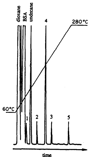
Fig. 6. Gas liquid chromatogram of the product mixture from \text{Me}(\text{Me}_2\text{SiO})_5\text{H} in dioxane at 35^{\circ}\text{C} in the presence of \text{CF}_3\text{SO}_3\text{H} ; [\text{CF}_3\text{SO}_3\text{H}]_0 = 2 \cdot 10^{-4} \text{ mol dm}^{-3} , [\text{4}]_0 = 0.5 \text{ mol dm}^{-3} , [\text{H}_2\text{O}]_0 = 1 \text{ mol dm}^{-3} , at 40% of the substrate conversion. The mixture was silylated with BSA. 1 – (\text{Me}_2\text{SiO})_4 (a product of side reaction: 4 \xrightarrow{\text{H}^+} (\text{Me}_2\text{SiO})_4 + \text{Me}_3\text{SiOH} ); 2 – \text{Me}(\text{Me}_2\text{SiO})_4\text{SiMe}_3 ; 3 – \text{Me}(\text{Me}_2\text{SiO})_6\text{SiMe}_3 ; 4 – \text{Me}(\text{Me}_2\text{SiO})_5\text{SiMe}_3 ; 5 – \text{Me}(\text{Me}_2\text{SiO})_9\text{SiMe}_3 .
