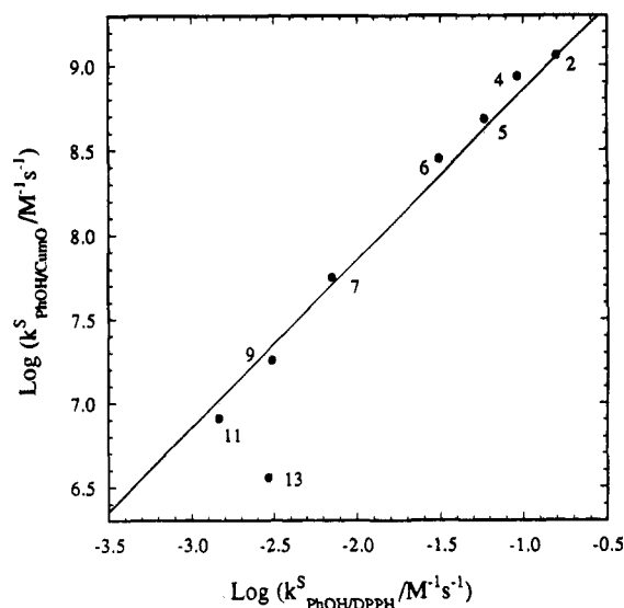
Figure 2. Plot of \log(k_{\text{PhOH/CumO}}^S) for the reaction of phenol with cumyloxyl radicals vs \log(k_{\text{PhOH/DPPH}}^S) for its reaction with 2,2-diphenyl-1-picrylhydrazyl radicals. The number beside each point corresponds to the solvent listed in Table 1 (plus 2% (CumO) 2 for the CumO • reactions). The line in this figure has a slope = 1.0.
