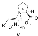
Figure 4. Plausible transition state V.
