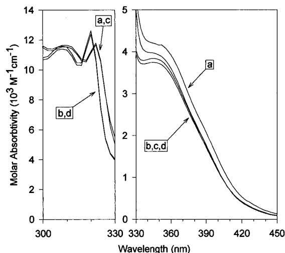
Figure 1. UV-visible absorption spectra of RePF 6 and ReBo . (a) ReBo /THF; (b) ReBo /CH 3 CN; (c) RePF 6 /THF; (d) RePF 6 /CH 3 CN. Spectra were obtained on solutions with 1.0 \times 10^{-4} M concentrations.
