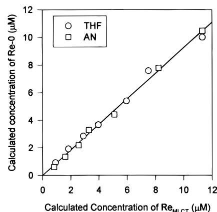
Figure 4. Plot of concentration of (\text{bpy}^{\bullet-})\text{Re}^{\text{I}}(\text{CO})_3(\text{py}) vs concentration of MLCT excited state, (\text{bpy}^{\bullet-})\text{Re}^{\text{I}}(\text{CO})_3(\text{py})^{\bullet+} , produced at laser powers ranging from 0.1 to 2.0 mJ/pulse. Circles and squares represent data for THF and \text{CH}_3\text{CN} solutions, respectively. The solid line represents the linear regression fit to the two data sets. The slope of the line is 0.92.
