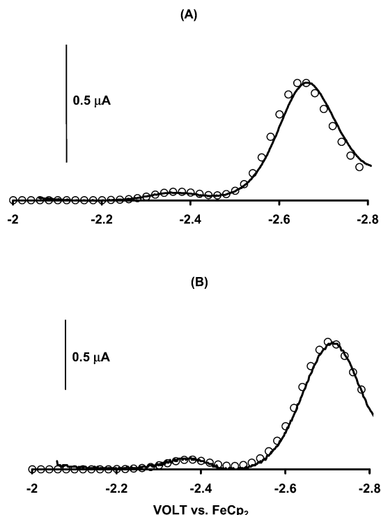
Figure 3. Square-wave voltammetry data for 0.72 mM 1 in THF/0.1 M [\text{NBu}_4][\text{CF}_3\text{SO}_3] at 296 K at a 2 mm glassy carbon electrode. Pulse height is 50 mV; pulse width is 2 mV. Experimental data are shown as solid lines; simulated, as open circles using parameters in Table 1. Frequency is 10 Hz (A); 100 Hz (B).
