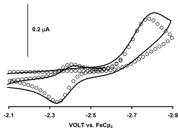
Figure 4. CV data for 0.72 mM 1 in THF/0.1 M [\text{NBu}_4][\text{CF}_3\text{SO}_3] at 296 K at a 2 mm glassy carbon electrode. Scan rate is 0.8 V \text{s}^{-1} . Experimental data are shown as solid lines; simulated, as open circles using parameters in Table 1.
