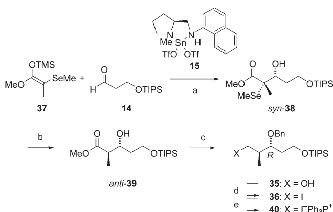
Scheme 6. Reagents and conditions: a) chiral \text{Sn}^{\text{II}} complex 15 , n\text{Bu}_3\text{SnF} , \text{CH}_2\text{Cl}_2 , -78^\circ\text{C} (57%, syn/anti 75:25, 95% ee for syn ); b) n\text{Bu}_2\text{BOTf} , i\text{Pr}_2\text{NEt} , \text{CH}_2\text{Cl}_2 , 0^\circ\text{C} ; then n\text{Bu}_3\text{SnH} , \text{Et}_3\text{B} , -78^\circ\text{C} (84%, anti/syn 90:10); c) i) \text{BnOC}(\text{CCl}_3)=\text{NH} , \text{TiOH} , \text{Et}_2\text{O} , 0^\circ\text{C} (85%); ii) \text{LiAlH}_4 , THF, 0^\circ\text{C} (98% from anti ); d) \text{I}_2 , \text{Ph}_3\text{P} , imidazole, benzene, RT (95%); e) \text{Ph}_3\text{P} , i\text{Pr}_2\text{NEt} , \text{CH}_3\text{CN} , reflux (quant).
