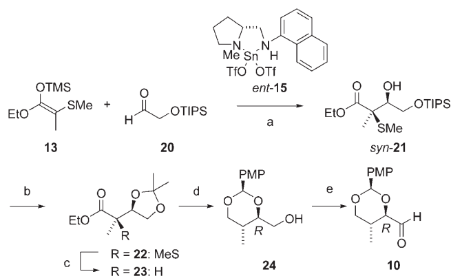
Scheme 4. Reagents and conditions: a) chiral \text{Sn}^{\text{II}} complex ent - 15 , n\text{Bu}_3\text{SnF} , \text{CH}_2\text{Cl}_2 , -78^\circ\text{C} (51%, syn/anti 81:19, 83% ee for syn ); b) i) tetrabutylammonium fluoride (TBAF), \text{AcOH} , THF, 0^\circ\text{C} (91% from syn ); ii) \text{Me}_2\text{C}(\text{OMe})_2 , \text{MsOH} , \text{CH}_2\text{Cl}_2 , RT (85%); c) n\text{Bu}_3\text{SnH} , AIBN, benzene, reflux (93%, anti/syn 88:12); d) i) \text{LiAlH}_4 , THF, 0^\circ\text{C} (82% from anti ); ii) pyridinium p -toluene sulfonate (PPTS), \text{MeOH} , reflux; iii) \text{PMPCH}(\text{OMe})_2 (PMP = 4-methoxyphenyl), PPTS, \text{CH}_2\text{Cl}_2 , RT (86%, two steps); e) \text{PhSNHtBu} , \text{NCS} , \text{K}_2\text{CO}_3 , MS 4Å, \text{CH}_2\text{Cl}_2 , RT (99%).
