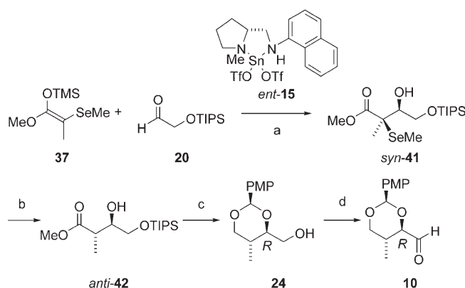
Scheme 7. Reagents and conditions: a) chiral Sn^{II} complex ent - 15 , nBu_3SnF , CH_2Cl_2 , -78^\circ C (54%, syn/anti 79:21, 88% ee for syn ); b) nBu_3BOTf , iPr_2NEt , CH_2Cl_2 , RT; then nBu_3SnH , Et_3B , -78^\circ C (77%, anti/syn 94:6); c) i) DIBAL, CH_2Cl_2 , 0^\circ C (80%); ii) PMPCH(OMe) 2 , CSA, CH_2Cl_2 , RT (84% from anti ); iii) TBAF, THF, 0^\circ C (95%); d) PhSNHtBu , NCS, K_2CO_3 , MS 4 Å, CH_2Cl_2 , RT (99%).
