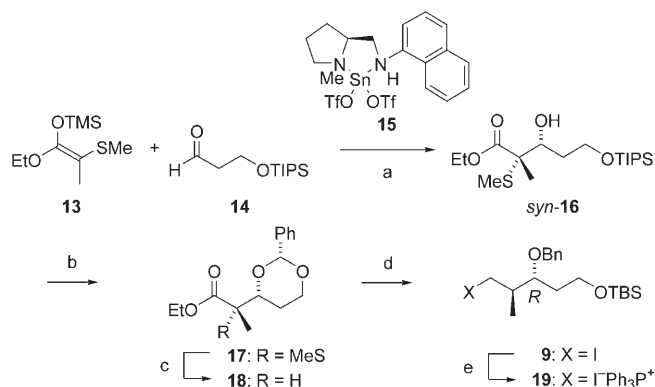
Scheme 3. Reagents and conditions: a) chiral \text{Sn}^{\text{II}} complex 15 , n\text{Bu}_3\text{SnF} , \text{CH}_2\text{Cl}_2 , -78^\circ\text{C} (64%, syn/anti 93:7, 87% ee for syn ); b) \text{PhCH}(\text{OEt})_2 , \text{TsOH} , \text{CH}_2\text{Cl}_2 , RT (77% from syn ); c) n\text{Bu}_3\text{SnH} , azobisisobutyronitrile (AIBN), benzene, reflux (quant, anti/syn 89:11); d) i) \text{LiAlH}_4 , THF, 0^\circ\text{C} (98% from anti ); ii) \text{I}_2 , \text{Ph}_3\text{P} , imidazole, benzene, RT (94%); iii) diisobutylaluminum hydride (DIBAL), \text{CH}_2\text{Cl}_2 , 0^\circ\text{C} (94%); iv) \text{TBSCl} , imidazole, DMF, RT (96%); e) \text{Ph}_3\text{P} , i\text{Pr}_2\text{NEt} , \text{CH}_3\text{CN} , reflux (84%).
