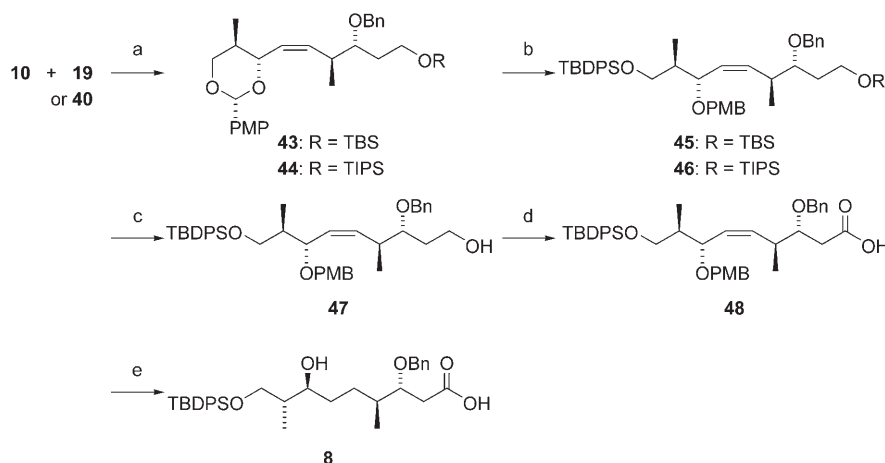
Scheme 8. Reagents and conditions: a) NaHMDS, toluene, -78^\circ C to RT (83% for 43 ; 88% for 44 ); b) i) DIBAL, CH_2Cl_2 , -5 or -10^\circ C (79% from 43 ; 86% from 44 ); ii) TBDPSCl, Et_3N , DMAP, CH_2Cl_2 , RT (91% for 45 ; 82% for 46 ); c) 1 M HCl, THF, RT (99% from 45 ; 95% from 46 ); d) i) DMP, CH_2Cl_2 , RT; ii) NaClO_2 , NaH_2PO_4 , 2-methyl-2-butene, tBuOH , H_2O , RT (94%, two steps) or TEMPO, NaClO_2 , NaClO , buffer, H_2O , CH_3CN , 35^\circ C (96%); e) i) CAN, H_2O , CH_3CN , 0^\circ C (94%); ii) H_2 , 10% Pd/C, Et_3N , MeOH, RT (87%).
