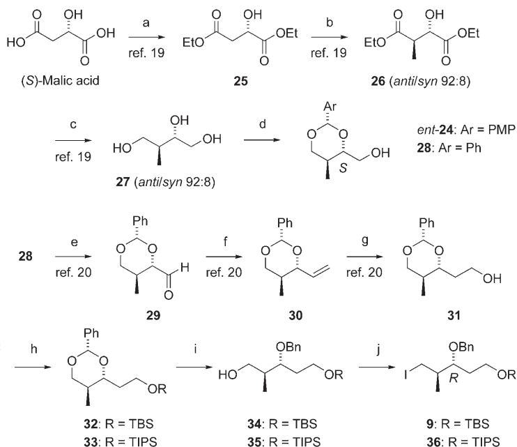
Scheme 5. Reagents and conditions: a) \text{H}_2\text{SO}_4 , \text{EtOH} , reflux (67%); b) \text{LDA} , \text{MeI} , THF, -78^\circ\text{C} (74%, anti/syn 92:8); c) \text{BH}_3\cdot\text{THF} , reflux (96%); d) \text{PMPCH}(\text{OMe})_2 , \text{CSA} , \text{CH}_2\text{Cl}_2 , RT (66% for ent - 24 ); \text{PhCH}(\text{OMe})_2 , \text{TsOH} , \text{CH}_2\text{Cl}_2 , RT (82% for 28 ); e) (\text{COCl})_2 , dimethylsulfoxide (DMSO), \text{Et}_3\text{N} , \text{CH}_2\text{Cl}_2 , -50^\circ\text{C} to RT (98%); f) \text{Br}\cdot\text{Ph}_3\text{P}^+\text{CH}_3 , \text{KHMDS} , THF, toluene, -78 to 0^\circ\text{C} (96%); g) 9-BBN, THF, 0^\circ\text{C} ; then \text{H}_2\text{O} , 3M \text{NaOH} , 35% \text{H}_2\text{O}_2 , RT (99%); h) \text{TBSCl} , imidazole, DMF, RT (87% for 32 ); \text{TIPSCl} , imidazole, DMF, RT (97% for 33 ); i) \text{BH}_3\cdot\text{SMe}_2 , \text{ZnEt}_2\cdot\text{OEt}_2 , THF, 50^\circ\text{C} (86% for 34 ); \text{DIBAL} , \text{CH}_2\text{Cl}_2 , 0^\circ\text{C} (90% for 35 ); j) \text{I}_2 , \text{Ph}_3\text{P} , imidazole, benzene, RT (90% for 9 ; 95% for 36 ).
