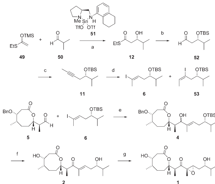
Scheme 10. Reagents and conditions: a) chiral Sn II complex 51 , n Bu 3 SnF, CH 2 Cl 2 , –78°C (65%, 94% ee ) or chiral Sn II complex 51 (20 mol%), CH 2 Cl 2 , –78°C (48%, 90% ee ); b) i) TBSCl, imidazole, DMF, RT (95%); ii) Et 3 SiH, 10% Pd/C, acetone, RT (88%); c) i) CBr 4 , PPh 3 , CH 2 Cl 2 , –78 to 0°C (86%); ii) n BuLi, THF, –78°C; then MeI, RT (91%); d) Cp 2 ZrHCl, benzene, sunlamp, 35°C; then I 2 , 7°C (72%, 6/53 70:30); e) 6 , n BuLi, Et 2 O, –78°C; then 5 (49%, \alpha/\beta = 57/43); f) i) tetra- n -propylammonium perruthenate (TPAP), NMO, MS 4 Å, CH 2 Cl 2 , 0°C (75%); ii) 46% HF, CH 3 CN, 0°C (91%); iii) BBr 3 , CH 2 Cl 2 , –95 to –45°C (76%); g) TBHP, VO(acac) 2 , CH 2 Cl 2 , 5–10°C (40% based on 70% conversion).
