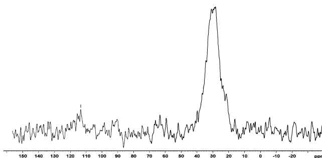
Figure 7. Solid-state 31 P spectrum of [Rh 2 (COD) 2 (dppm)(μ 2 -Cl)]-BF 4 ( 1 ) entrapped in silica.
