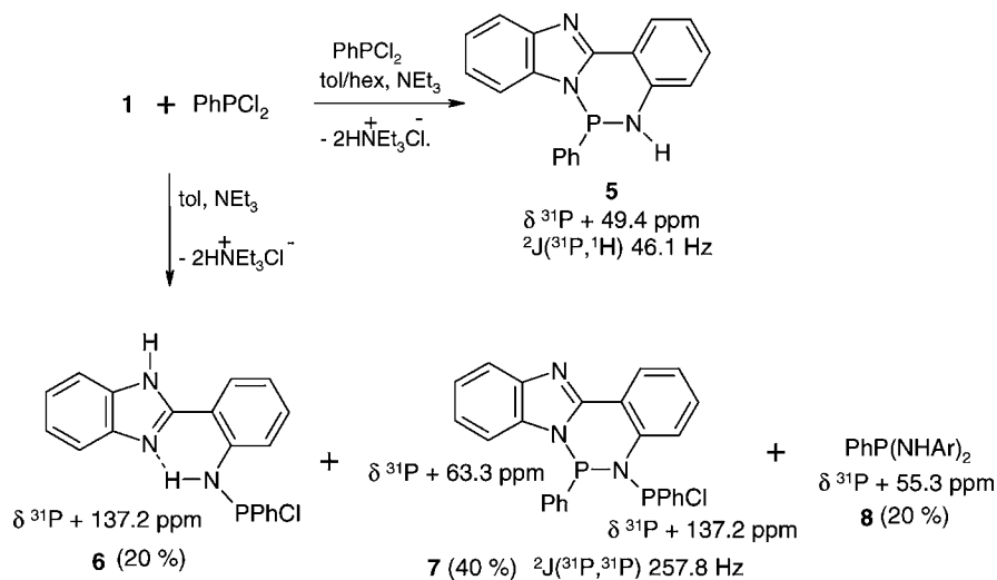
SCHEME 3 Synthesis and ^{31}\text{P} NMR data of compounds 5–7.
