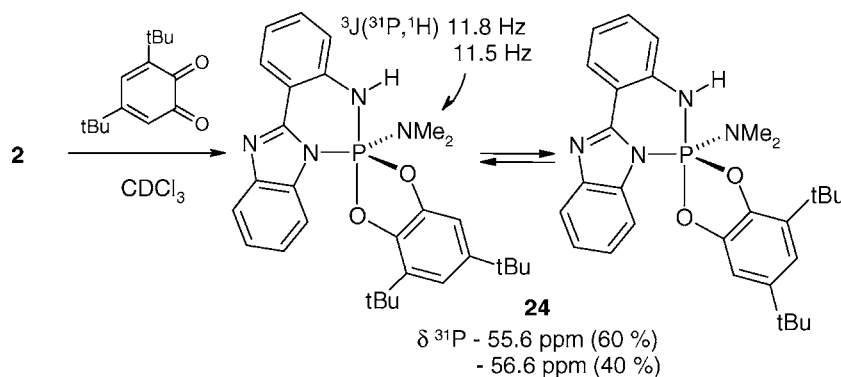
SCHEME 8 Synthesis and ^{31}\text{P} NMR data of spirophosphoranes 24 .
