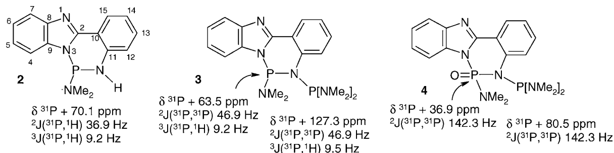
SCHEME 2 ^{31}\text{P} NMR data of compounds 2–4.
