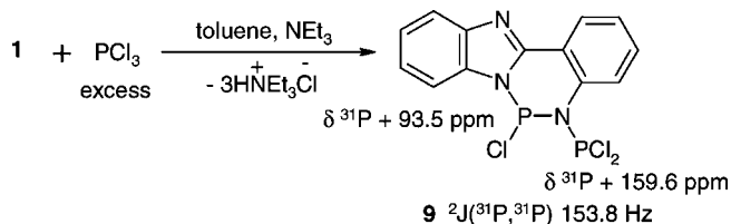
SCHEME 4 Synthesis and ^{31}\text{P} NMR data of compound 9.
