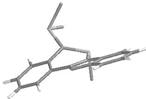
FIGURE 1 Model of compound 9 calculated using the PM3 program [25].
