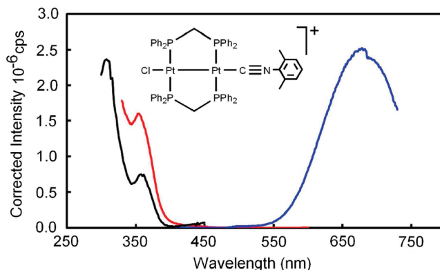
Figure 5. Absorption (black), excitation (red), and emission (blue) spectra of 3a' in PrCN at 77 K. \lambda_{\text{exc}} = 370 nm.
