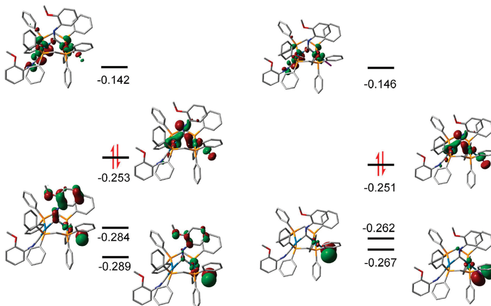
Figure 9. MO pictures of the LUMO, HOMO, HOMO–1, and HOMO–2 of 11a (right) and 11b (left).
