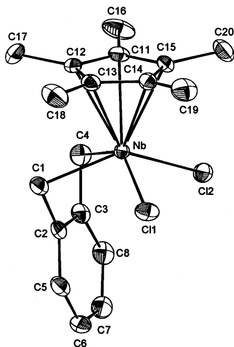
Fig. 1. ORTEP drawing of \text{Cp}^*\text{Nb}\{o\text{-(CH}_2\text{)}_2\text{C}_6\text{H}_4\}\text{Cl}_2 ( 1 ) with the numbering scheme.
