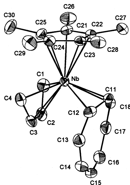
Fig. 3. ORTEP drawing of \text{Cp}^*\text{Nb}(\eta^4\text{-C}_4\text{H}_6)(\eta^3\text{-C}_8\text{H}_8) ( 16 ) with the numbering scheme.
