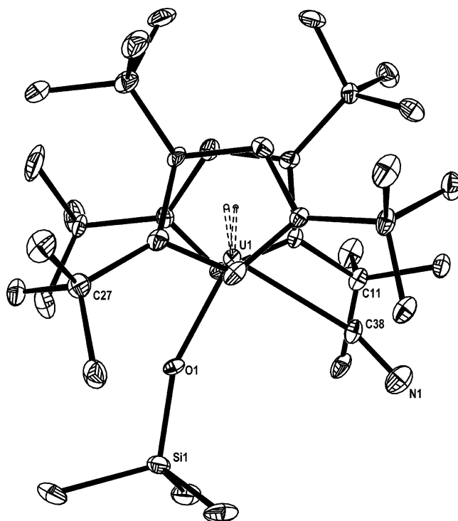
Figure 8. ORTEP drawing of [\eta^5\text{-1,2,4-(Me}_3\text{C)}_3\text{C}_5\text{H}_2]_2\text{U(OSiMe}_3\text{)(CN)} ( 14 ) with 35% thermal ellipsoids.
