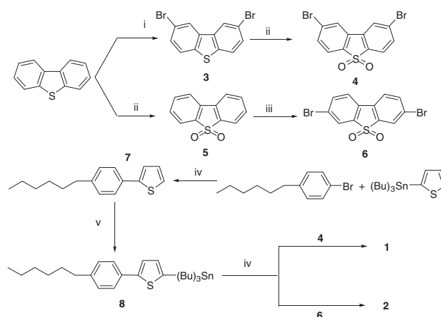
Scheme 2. Reaction conditions; i) Br 2 , CH 3 COOH, 25 °C, 2 h, 115 °C, 5 h; ii) H 2 O 2 , CH 3 COOH, 110 °C, 4 h; iii) NBS, H 2 SO 4 , 25 °C, 12 h; iv) DMF, [Pd(PPh 3 ) 4 ], 100 °C, 40 h; v) n -BuLi, −78 °C, 1 h, then, (Bu) 3 SnCl, 25 °C, 12 h.
