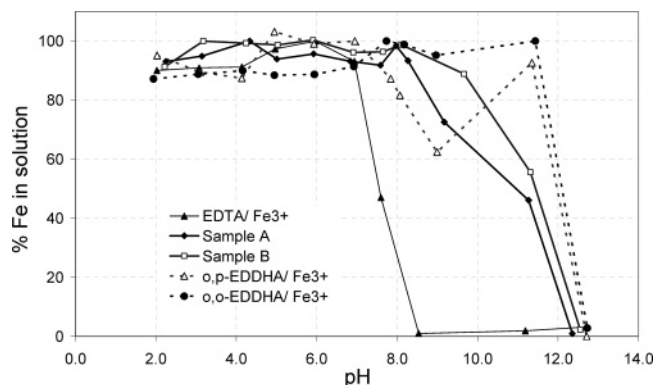
Figure 5. Percent of soluble Fe recovered at different pHs in 10 mM \text{Ca}^{2+} solution.
